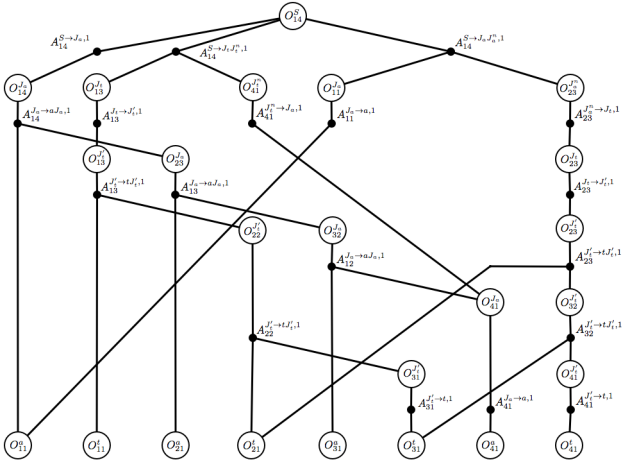
Fig. 2 DAG \Gamma for grammar from Example 4
