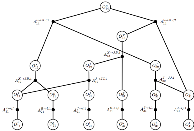
Fig. 1 DAG \Gamma for grammar from Example 2 on word of length 4
