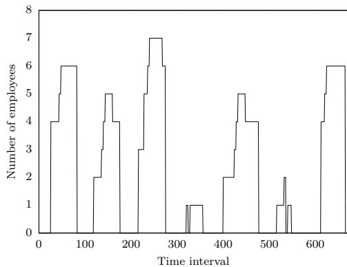
Figure 4: Smooth demand pattern
