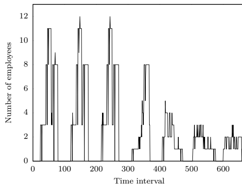
Figure 5: Erratic demand pattern
