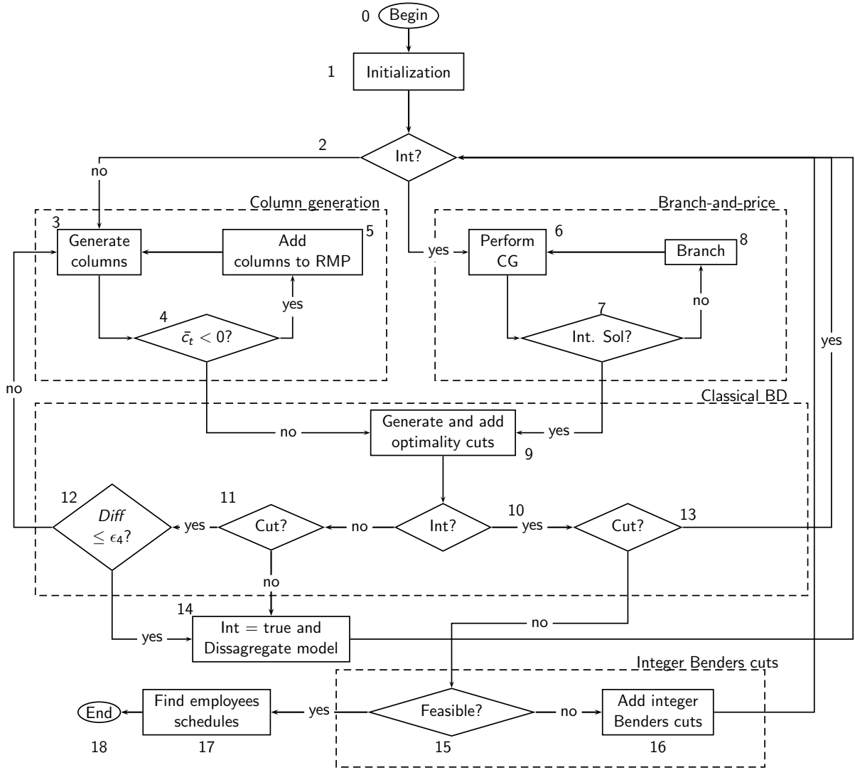
Figure 3: Flow chart of the BD/CG algorithm for the MATSP
